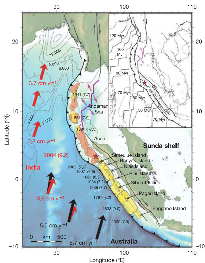
Figure 1 | Tectonic setting and ruptures of major interplate earthquakes along the Sunda megathrust. The yellow patches are estimated rupture areas of known large subduction events between 1797 and 2004 (refs 7, 9, 20). Orange patches depict the 2004 Sumatra–Andaman rupture where slip was 5 m or more. Tectonic features are simplified from Curray 43 and Natawidjaja et al. 20 . The boundary between Australia and India is a diffuse plate boundary between \sim 5^\circ S and 8^\circ N (ref. 44). Plate velocities of Australia (black arrows) and India (red arrows) relative to Sunda were computed from a regional kinematic model 1 . Dashed lines are contours of sediment thickness at intervals of 2,000 m. The inset shows that the age of the sea floor increases northwards, from \sim 50 Myr in the epicentral area to 80–120 Myr at the latitude of the Andaman islands.
