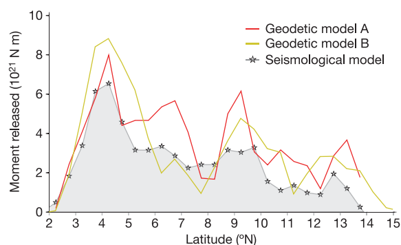
Figure 4 | Latitudinal variations of scalar moments as determined from seismic waveforms (model III of ref. 14) and from geodetic data. Moment released per half degree in latitude. Both geodetic models imply a rougher slip distribution than the seismic model. The total moment for geodetic model A ( 8.78 \times 10^{22} \text{ N m} ) exceeds the seismic moment by 30\% \pm 12\% . This excess presumably reflects afterslip during the 30 days following the main shock.
