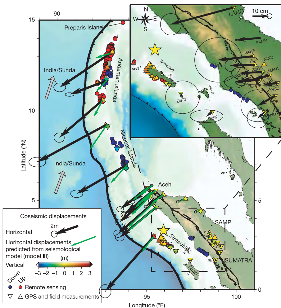
Figure 2 | Comparison of near-field geodetic measurements (black arrows) with predictions (green arrows) of the seismic model III of ref. 14. This comparison suggests that the geodetic data require more slip, a different spatial distribution of slip, or both. The inset shows a close-up of the Simeulue area. Horizontal displacements are shown with 95% confidence ellipses (see tables in Supplementary Information 1). Vectors in the Andaman and Nicobar islands are from CESS ( http://www.seires.net/content/view/123/52/ ).
