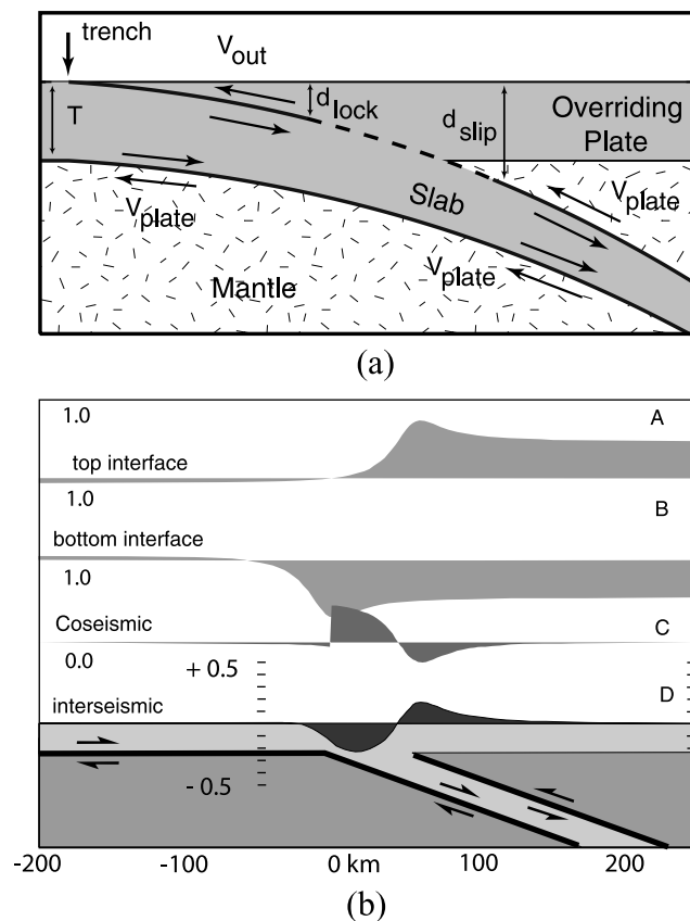
Figure 18. (a) Sketch showing the parameters of an idealized elastic dislocation model of deformation at a subduction zone. Dark lines are slipping interface. Dashed line is a locked patch or patch that slips during the event [after Sieh et al. , 1999]. (b) An elastic dislocation model of an earthquake cycle. Dark bold line is interface slips at the plate rate. Panels A and B show contributions to vertical motion from individual sources. Panel D shows the combined vertical motions from top and bottom of the slab. Note that motions due to slip on the top and the bottom interfaces are nearly mirror images of each other. So, in steady state subduction they nearly cancel one another. Panel C shows vertical motion during a seismic event, which nearly mirrors that of the interseismic period.
