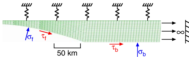
Figure 1. Portion of finite element mesh used in stress computations with applied boundary conditions.
