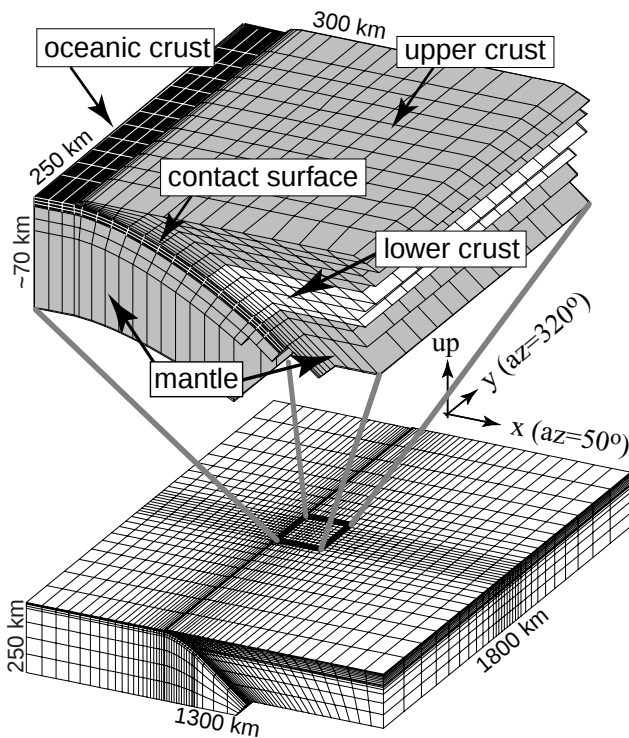
Figure 2. FEM configuration, FEM_C . The problem domain is tessellated into 24,750 three-dimensional elements. The expanded ~70 km-thick portion of the near-field region displays the heterogeneous material property distribution and subduction zone geometry.
