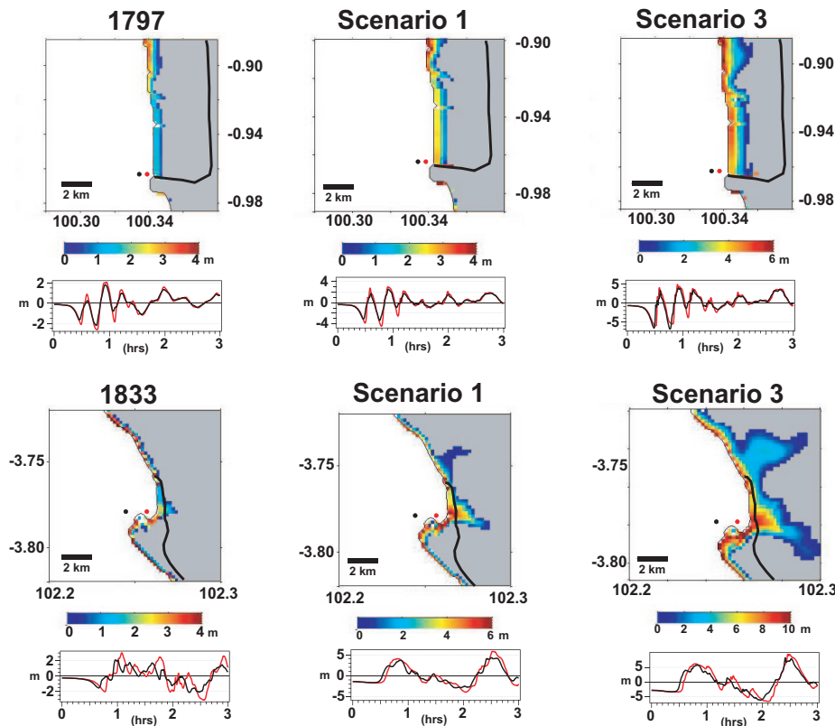
Fig. 3. Computed tsunami flow depths and inundations over local coastal topography near Padang ( Upper ) and Bengkulu ( Lower ) for a subset of the model scenarios. Pixel dimension is \approx 200 \times 200 m. In each panel, tsunami time series begin at the time of rupture and are for offshore locations at 5 m (red dot) and 10 m (black dot). Solid black line represents the extent of densely populated urban areas. The simulations of 1797 and 1833 tsunamis are consistent with sparse historical accounts. Simulations of plausible future events show that both Padang and Bengkulu could be seriously impacted by future tsunamis. The effects at Bengkulu, unprotected by offshore islands, will likely be more severe than at Padang.
