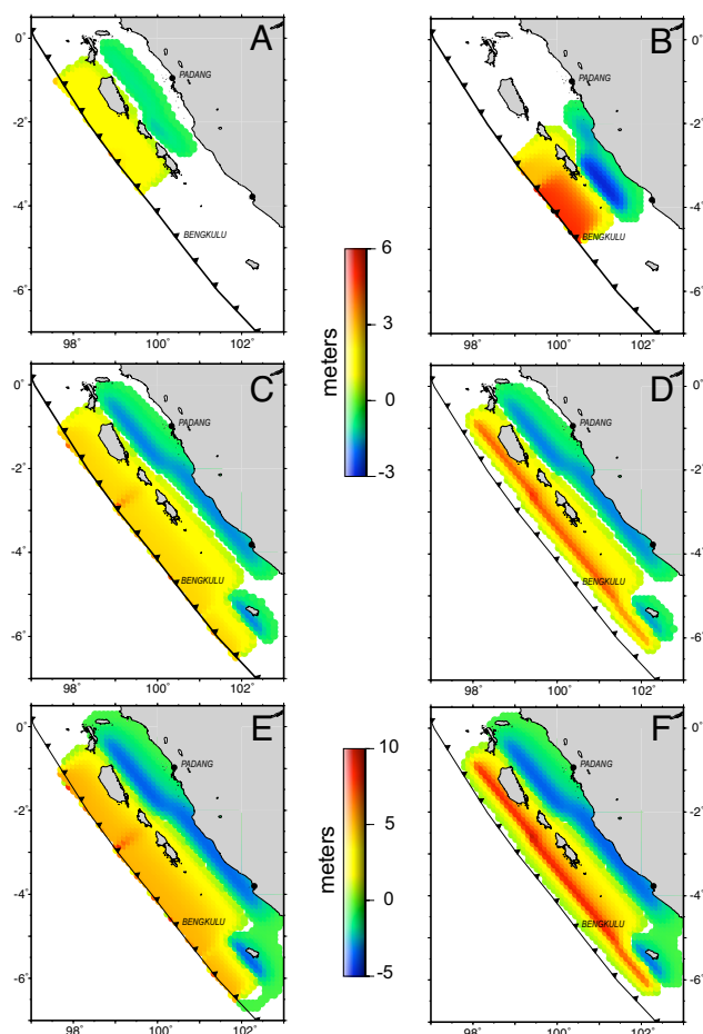
Fig. 2. Vertical deformation patterns produced by the six megathrust ruptures used in this study. (A and B) Effects of the 1797 (A) and 1833 (B) ruptures are from Natawidjaja et al. (5). (C) In scenario 1, uniform slip of 10 m extends to trench. (D) In scenario 2, uniform slip of 10 m extends up-dip only to a depth of 15 km. (E) In scenario 3, uniform slip of 20 m extends to trench. (F) In scenario 4, uniform slip extends up-dip only to a depth of 15 km.
