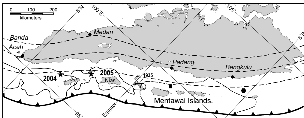
Fig. 1. Map of recent and plausible future sources of Sumatran tsunamis. Barbed line is the seafloor trace of the Sunda megathrust, which dips beneath Sumatra. The roughly parallel dashed lines are the 50-, 100-, and 200-km iso-depth contours of the Sunda megathrust (1). Stars and surrounding irregular lines represent the epicenters and ruptures of the tsunamigenic December 2004 and March 2005 earthquakes. Slip was >1 m inside the lines. The dashed line south of the Equator is the locked part of the megathrust that is likely to be the source of the next great earthquake. The small, rectangular patch is the source region of the M_w 7.7 earthquake of 1935, where great ruptures do not occur (2, 3). The box is the epicenter of the April 10, 2005 ( M_w 6.7 ) aftershock.
