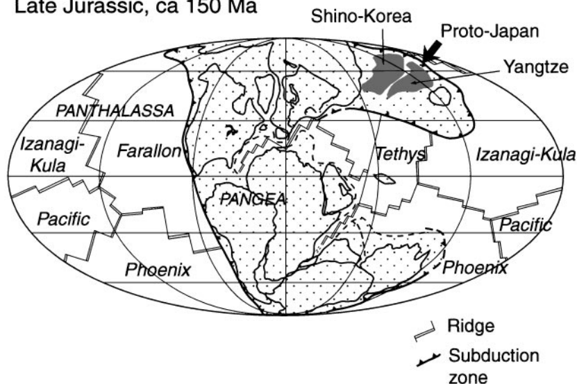
Figure 12 Paleogeography of Pangea and Panthalassa and the possible location of proto-Japan in the late Permian (~255 Ma) and late Jurassic (~150 Ma). Note that proto-Japan evolved from the Tethys-Panthalassa (Pacific) corner. (After Isozaki 1997.)
