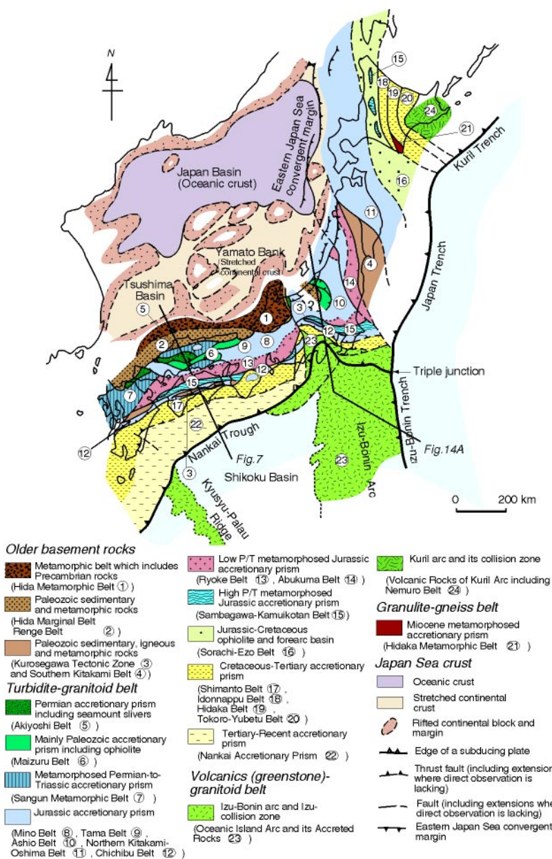
Figure 6 Basement geology map of the Japanese arc system, excluding the distribution of granitic rocks shown in Figure 9. See text for explanation of geological classification. (After Taira et al 1989, 1998, Maruyama 1997, and Isozaki 1996.)
