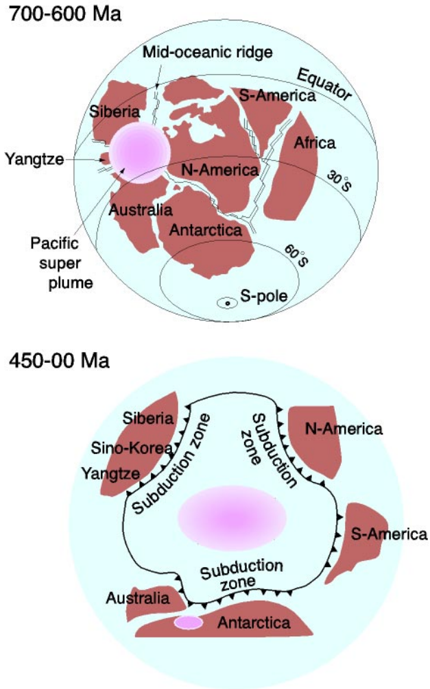
Figure 13 A schematic model showing the breakup of a Late Proterozoic supercontinent by a Pacific super plume and subsequent evolution of the Pacific rim. (After Maruyama 1997.)
