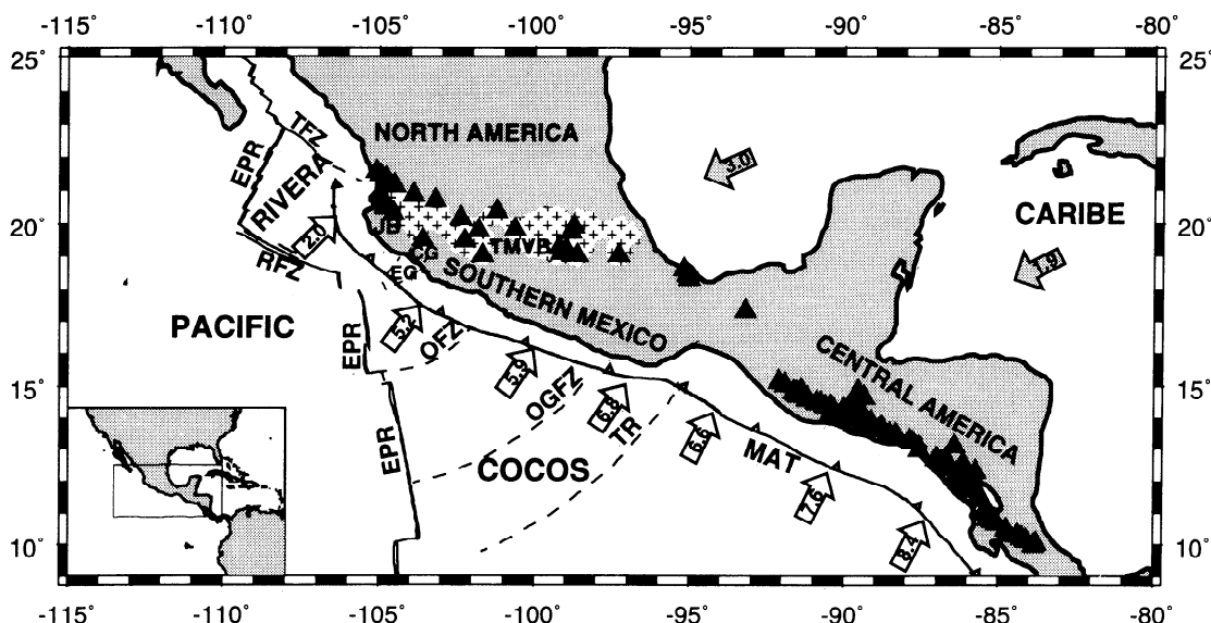
Figure 1. General tectonic setting of the study area. Five lithospheric plates are shown: Pacific, Rivera, Cocos, North America, and Caribbean. Relative convergence rates (cm/yr) between the oceanic and continental plates are indicated by open arrows, and absolute motions of the upper plates relative to a hot spot frame of reference are shown by shaded arrows. The abbreviations are EPR, East Pacific Rise; TFZ, Tamayo Fracture Zone; RFZ, Rivera Fracture Zone; OFZ, Orozco Fracture Zone; OGFZ, O'Gorman Fracture Zone; TR, Tehuantepec Ridge; MAT, Middle American Trench; JB, Jalisco Block; CG, Colima Graben; EG, El Gordo Graben. Solid triangles indicate Quaternary volcanism, and the crossed area indicates the Trans-Mexican Volcanic Belt (TMVB).
